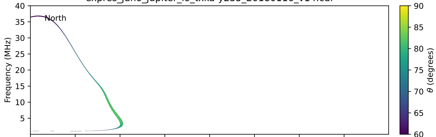
expres_juno_jupiter_io_txka-y235_20180116_v14.cdf
