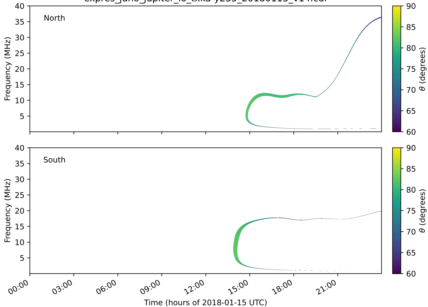
expres_juno_jupiter_io_txka-y235_20180115_v14.cdf
