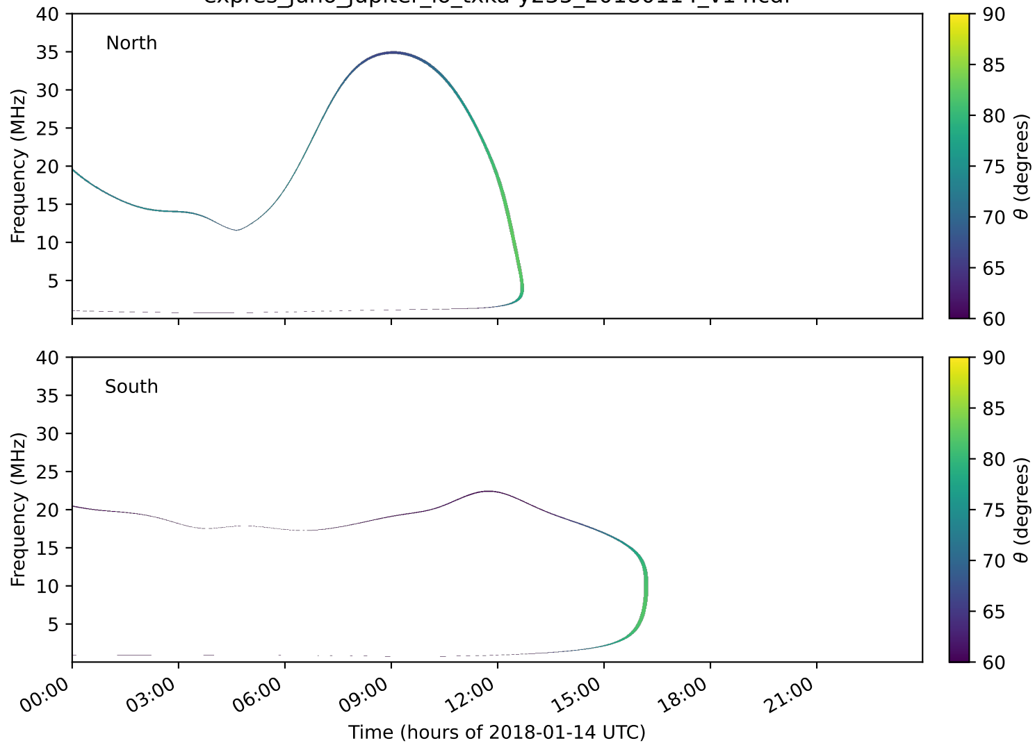
expres_juno_jupiter_io_txka-y235_20180114_v14.cdf
