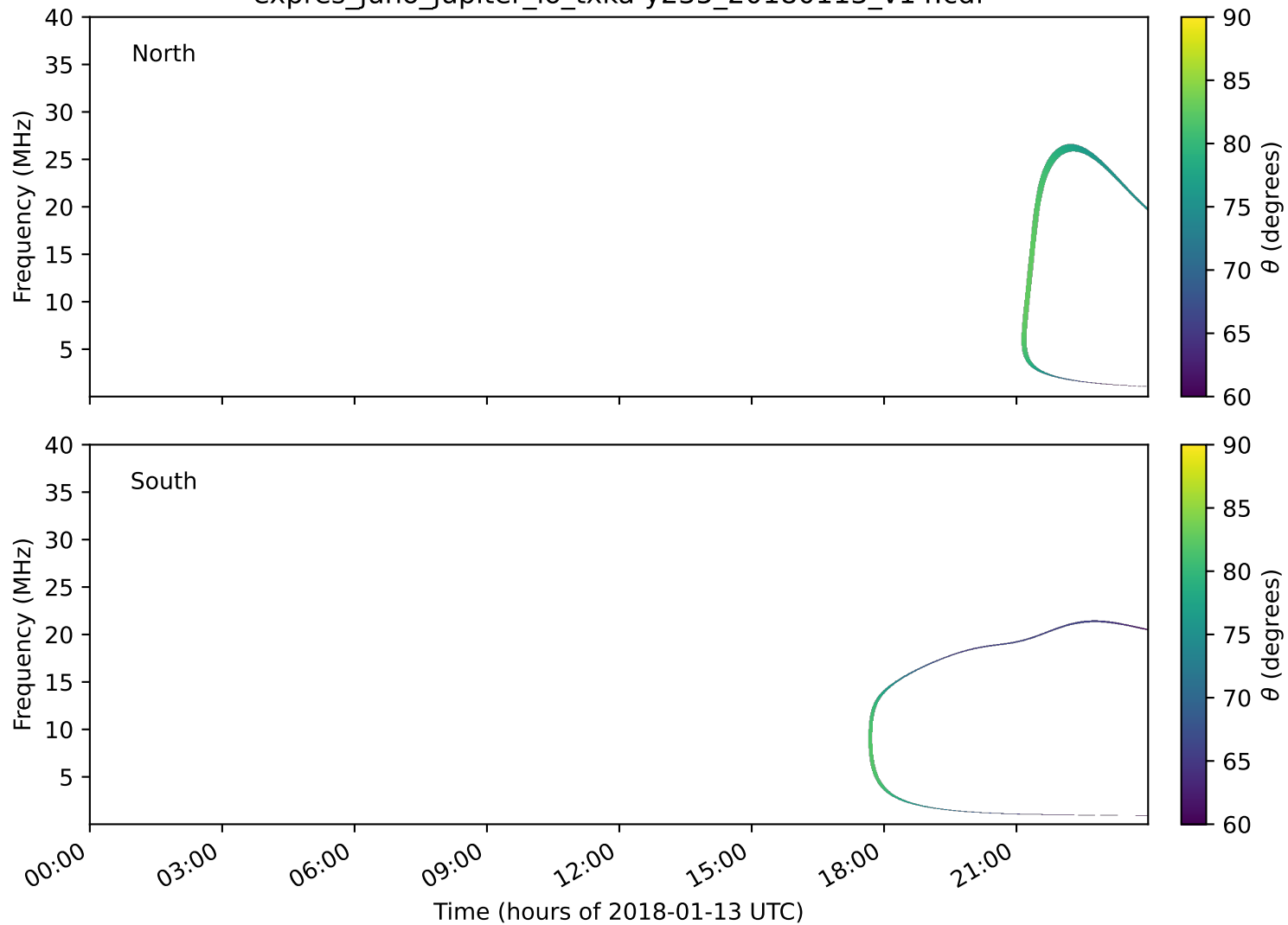
expres_juno_jupiter_io_txka-y235_20180113_v14.cdf
