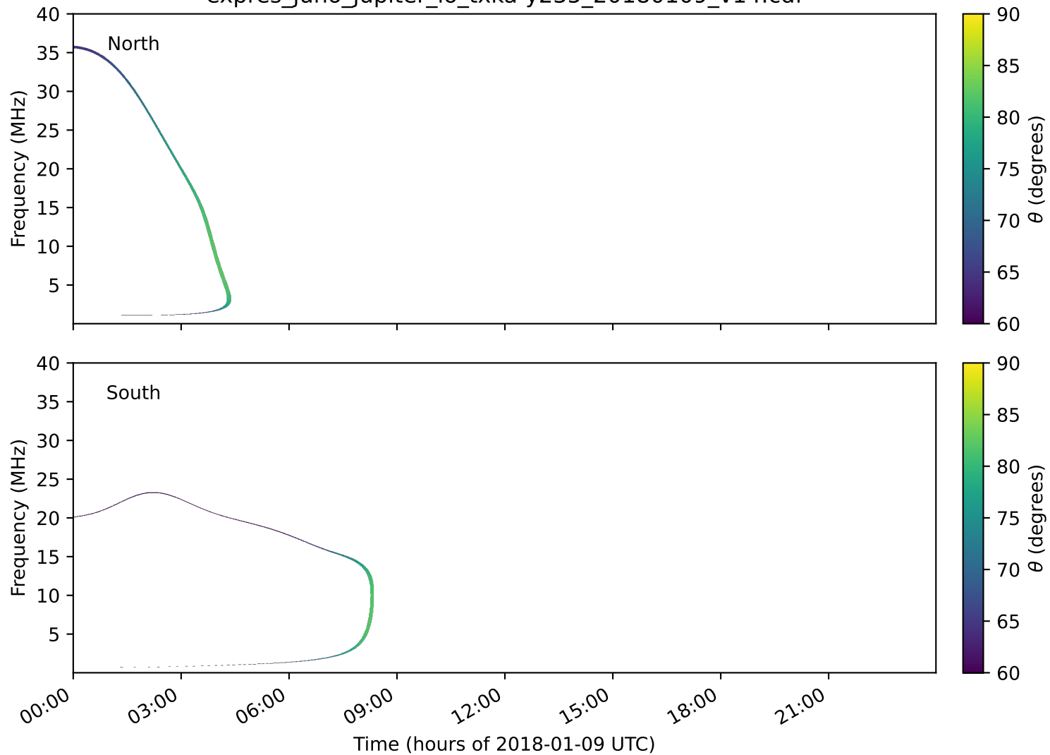
expres_juno_jupiter_io_txka-y235_20180109_v14.cdf
