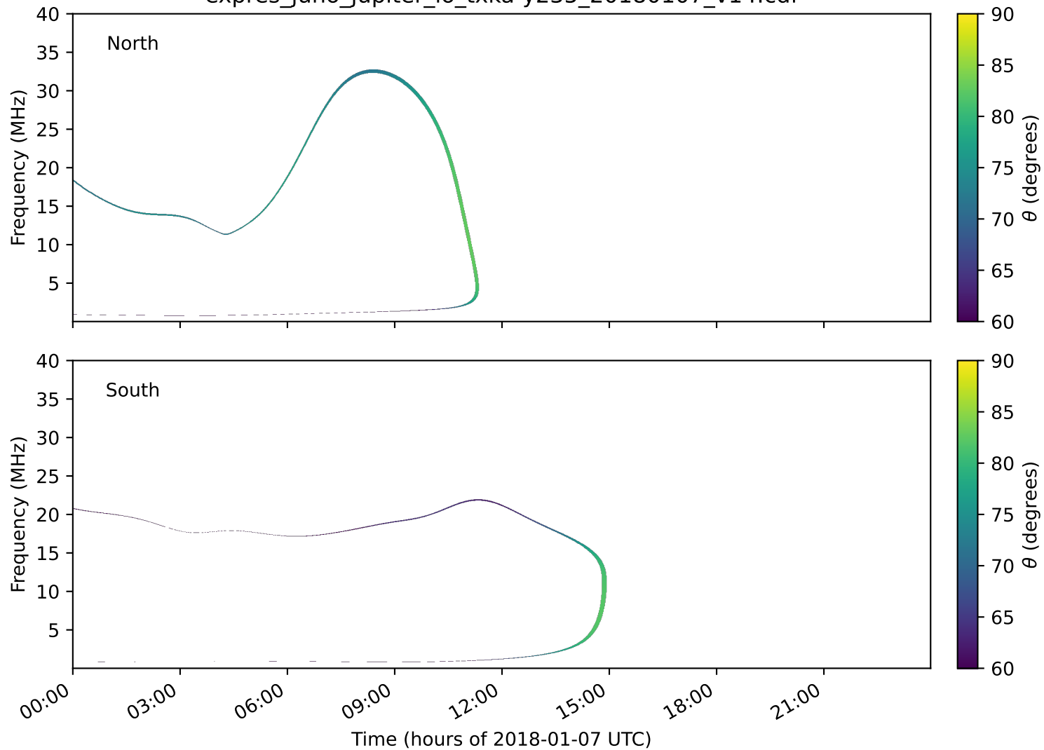
expres_juno_jupiter_io_txka-y235_20180107_v14.cdf
