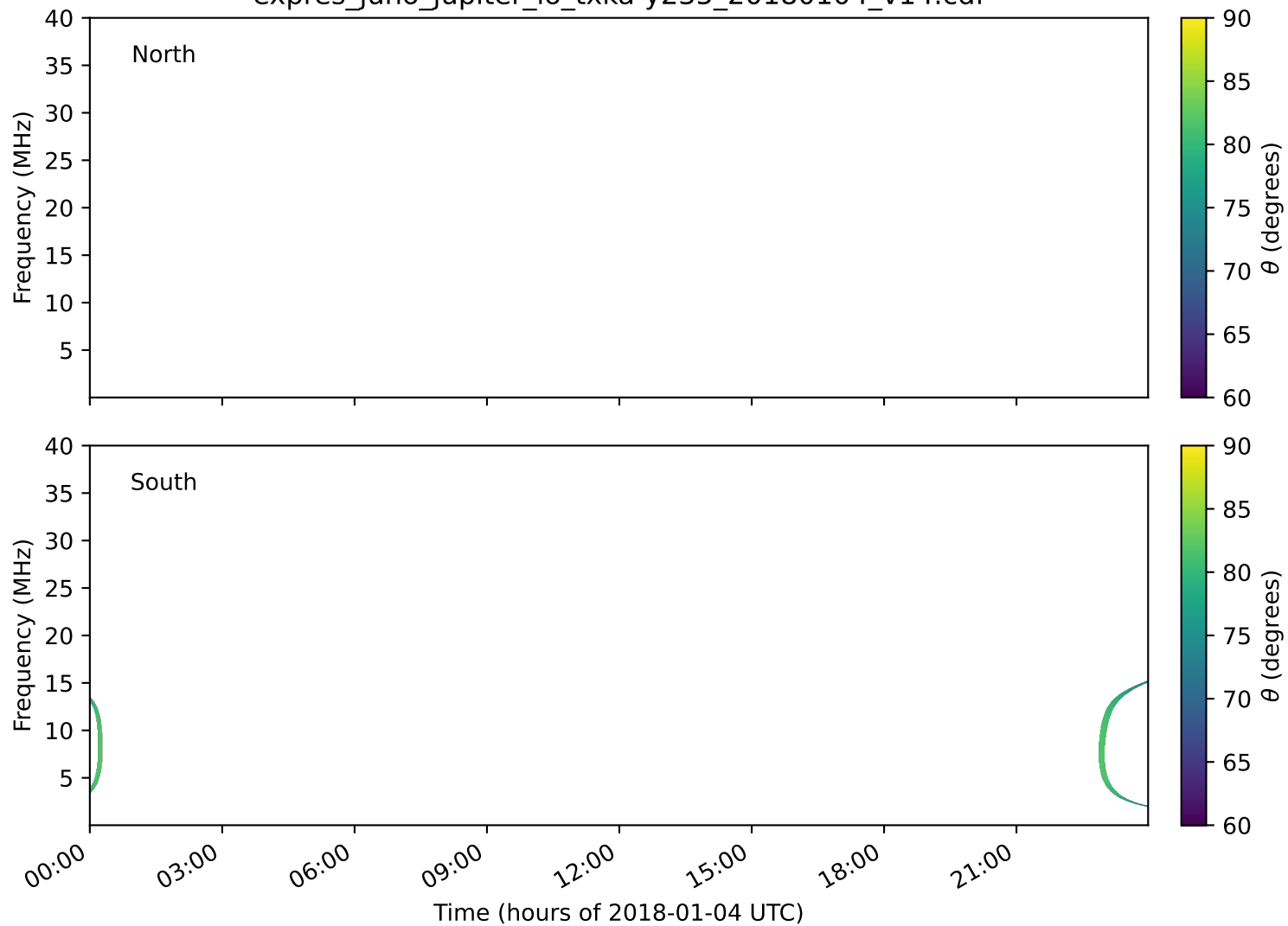
expres_juno_jupiter_io_txka-y235_20180104_v14.cdf
