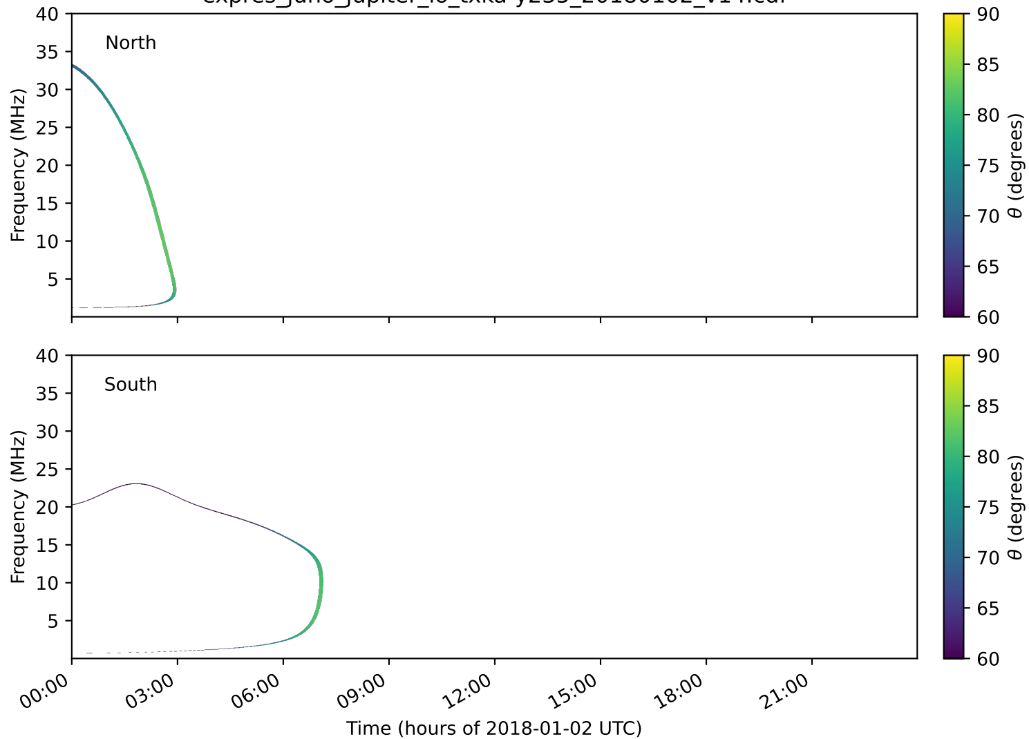
expres_juno_jupiter_io_txka-y235_20180102_v14.cdf
