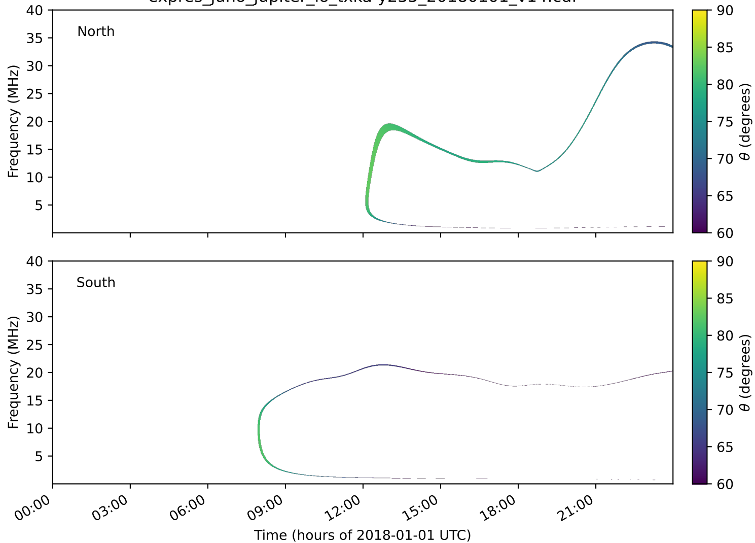
expres_juno_jupiter_io_txka-y235_20180101_v14.cdf
