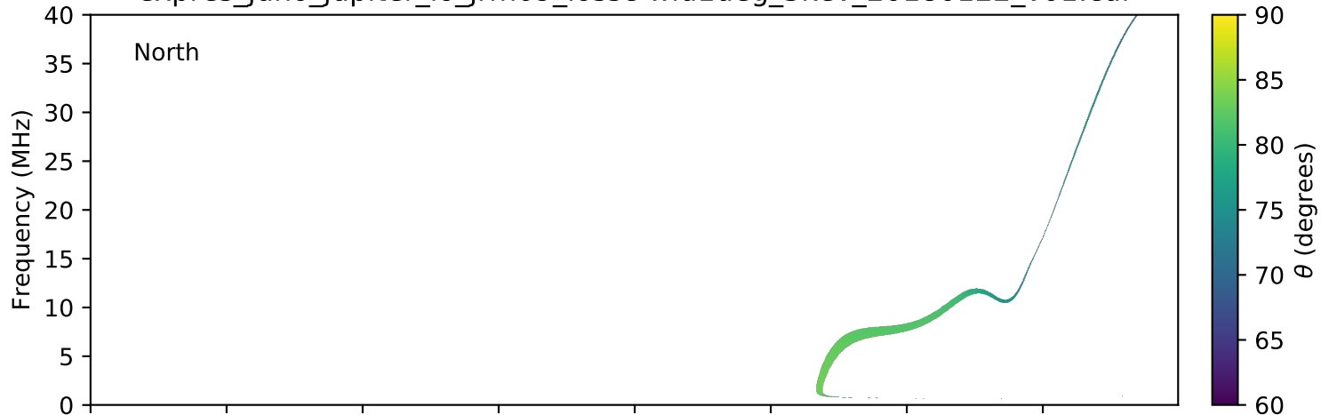
expres_juno_jupiter_io_jrm09_lossc-wid1deg_3kev_20180122_v01.cdf
