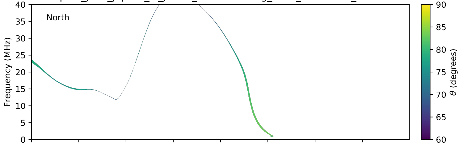
expres_juno_jupiter_io_jrm09_lossc-wid1deg_3kev_20180121_v01.cdf
