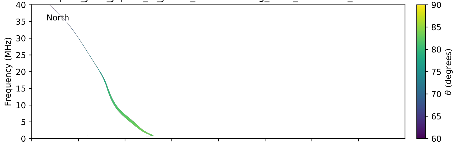
expres_juno_jupiter_io_jrm09_lossc-wid1deg_3kev_20180116_v01.cdf
