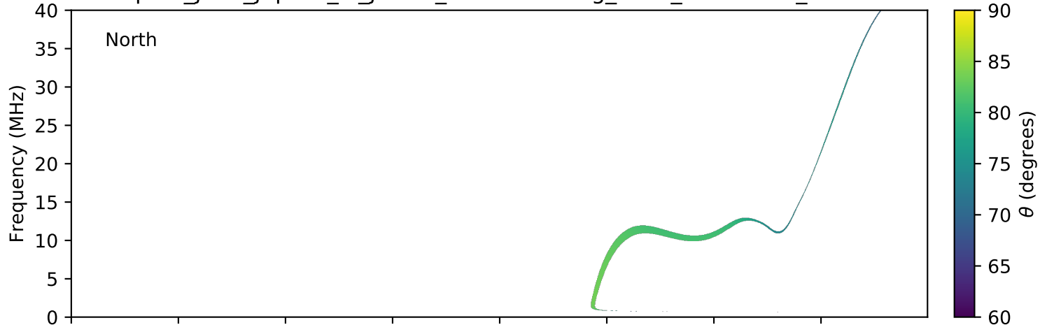
expres_juno_jupiter_io_jrm09_lossc-wid1deg_3kev_20180115_v01.cdf
