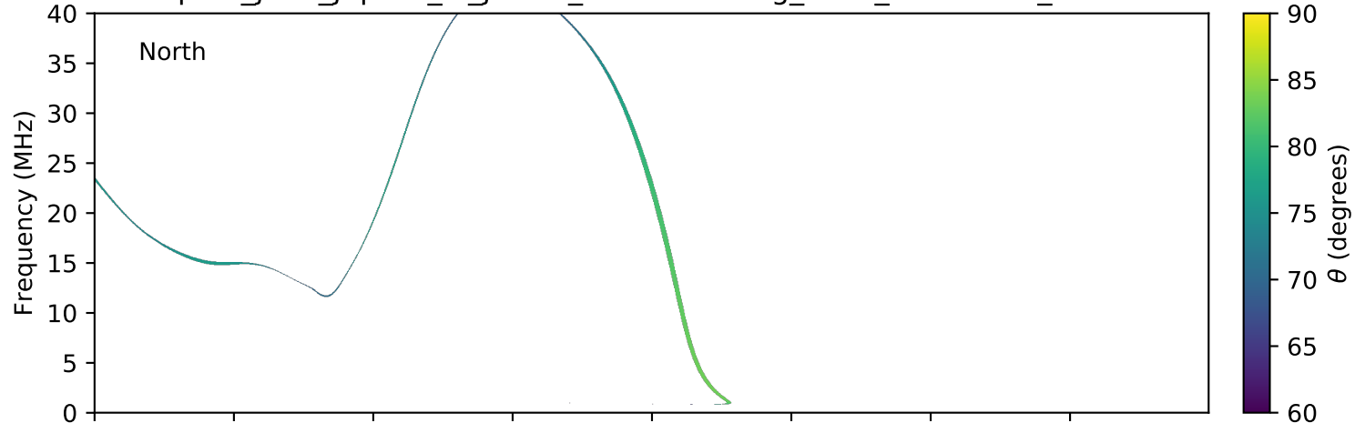
expres_juno_jupiter_io_jrm09_lossc-wid1deg_3kev_20180114_v01.cdf
