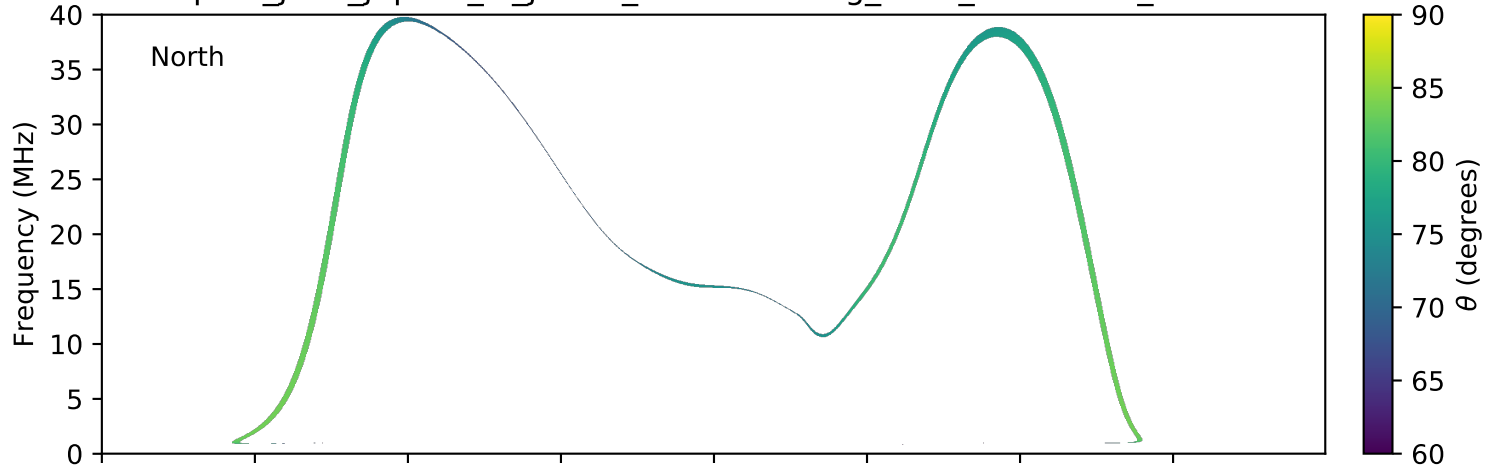
expres_juno_jupiter_io_jrm09_lossc-wid1deg_3kev_20180112_v01.cdf
