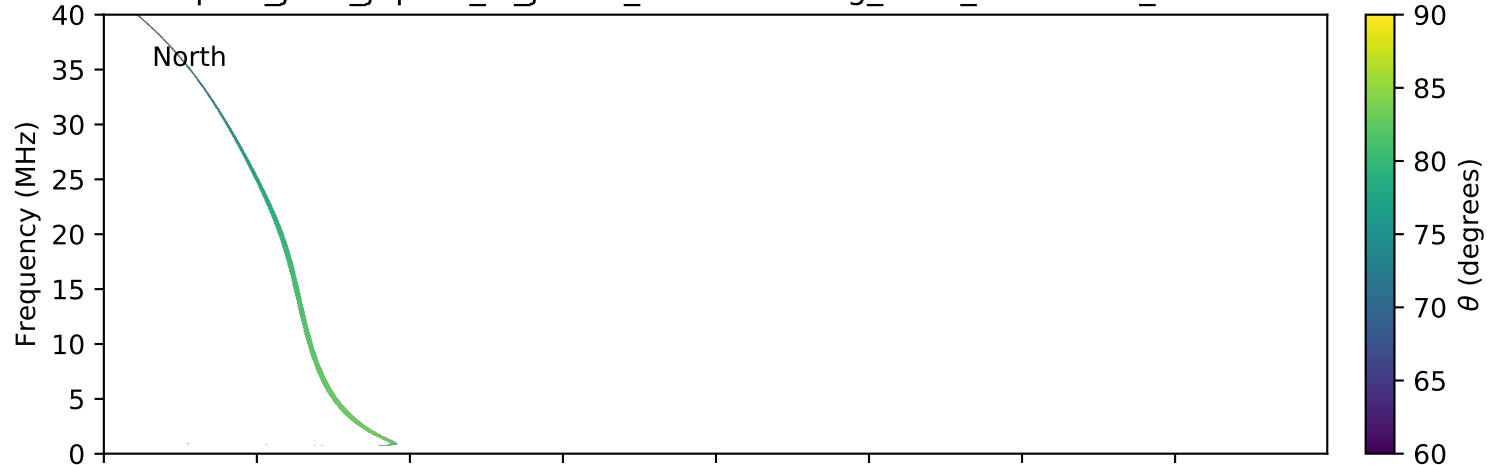
expres_juno_jupiter_io_jrm09_lossc-wid1deg_3kev_20180109_v01.cdf
