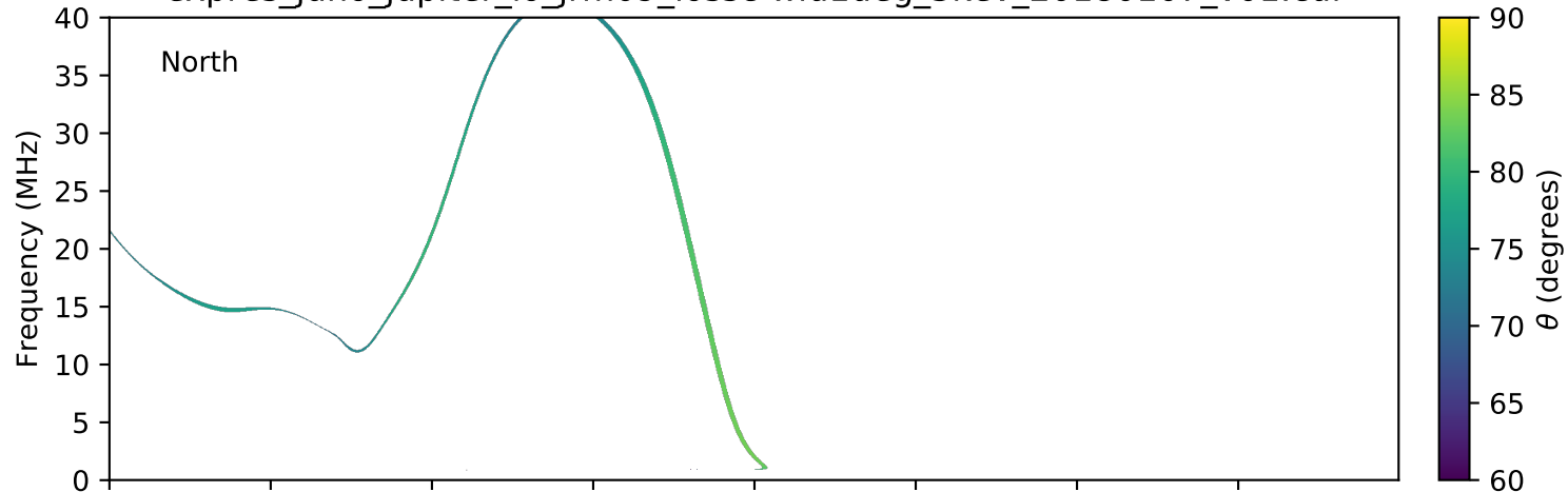
expres_juno_jupiter_io_jrm09_lossc-wid1deg_3kev_20180107_v01.cdf
