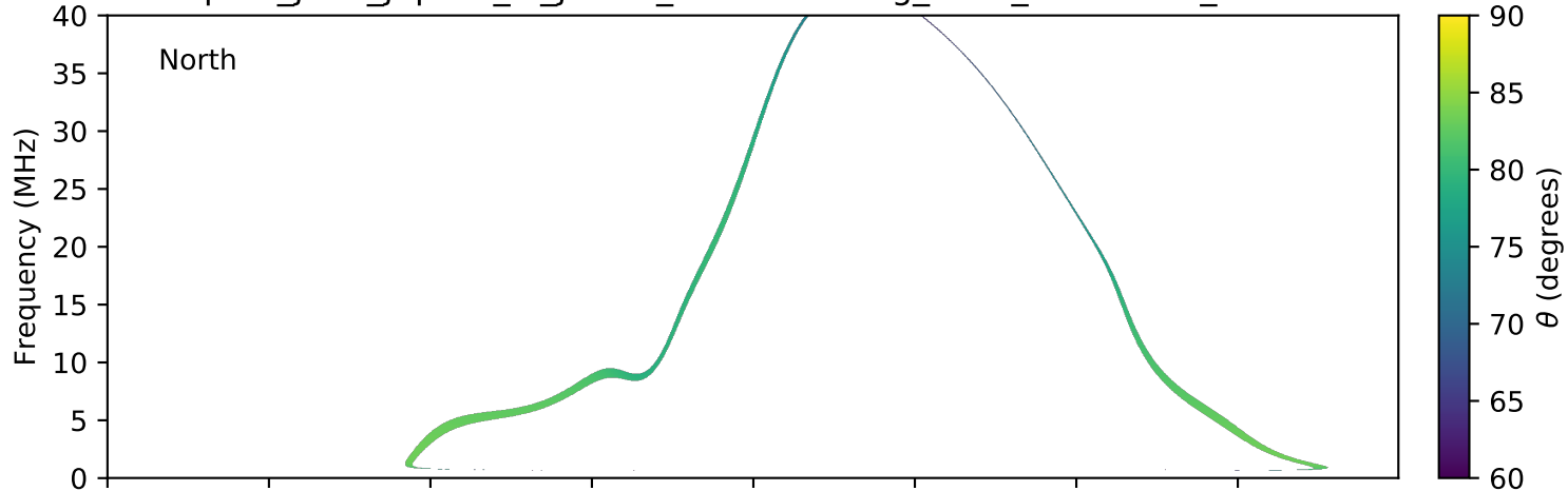
expres_juno_jupiter_io_jrm09_lossc-wid1deg_3kev_20180103_v01.cdf
