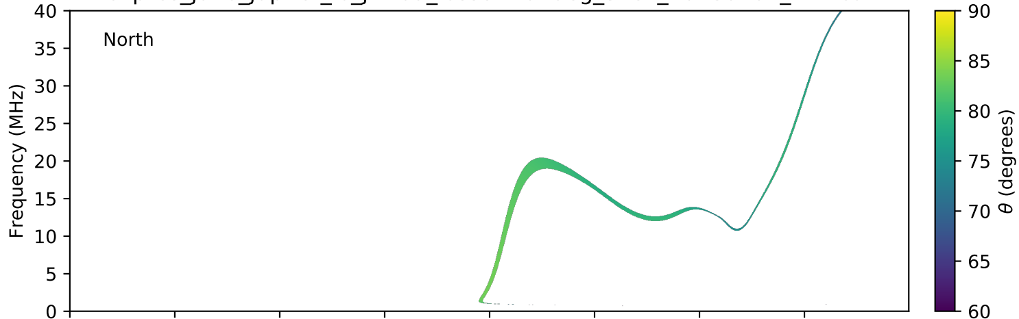
expres_juno_jupiter_io_jrm09_lossc-wid1deg_3kev_20180101_v11.cdf
