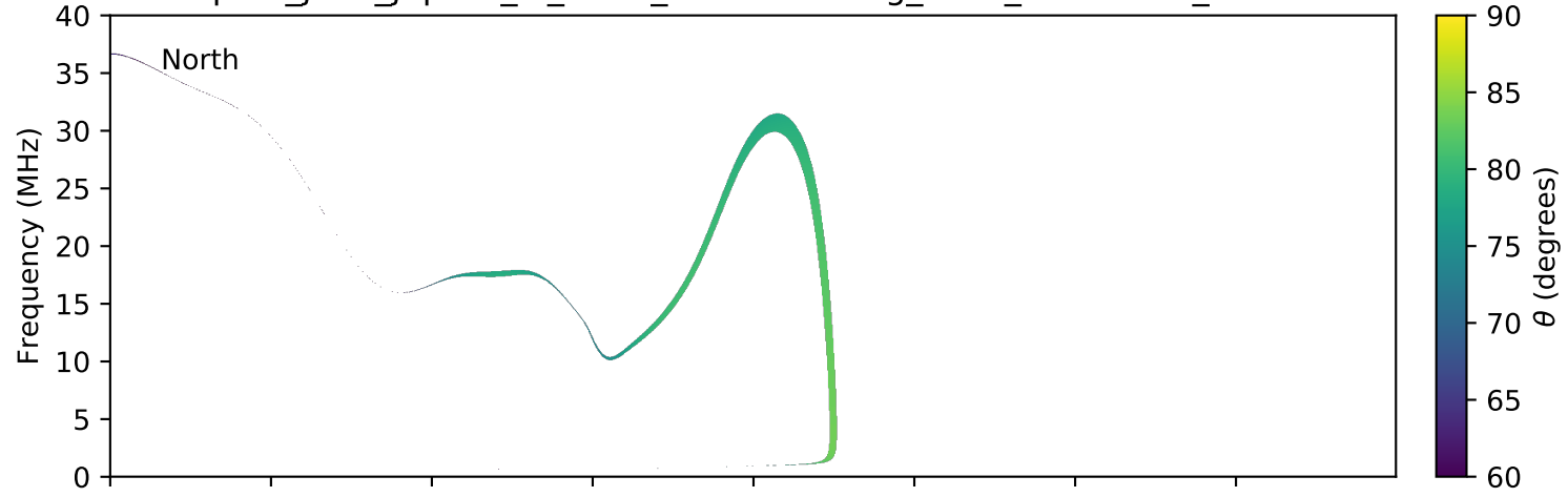
expres_juno_jupiter_io_isaac_lossc-wid1deg_3kev_20180130_v01.cdf
