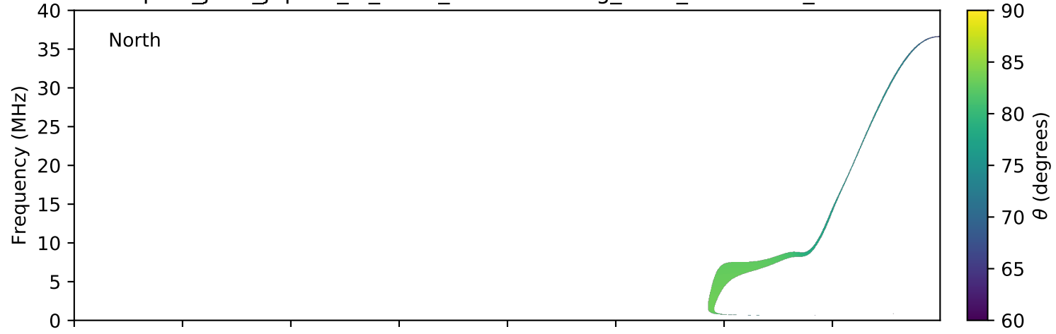
expres_juno_jupiter_io_isaac_lossc-wid1deg_3kev_20180129_v01.cdf
