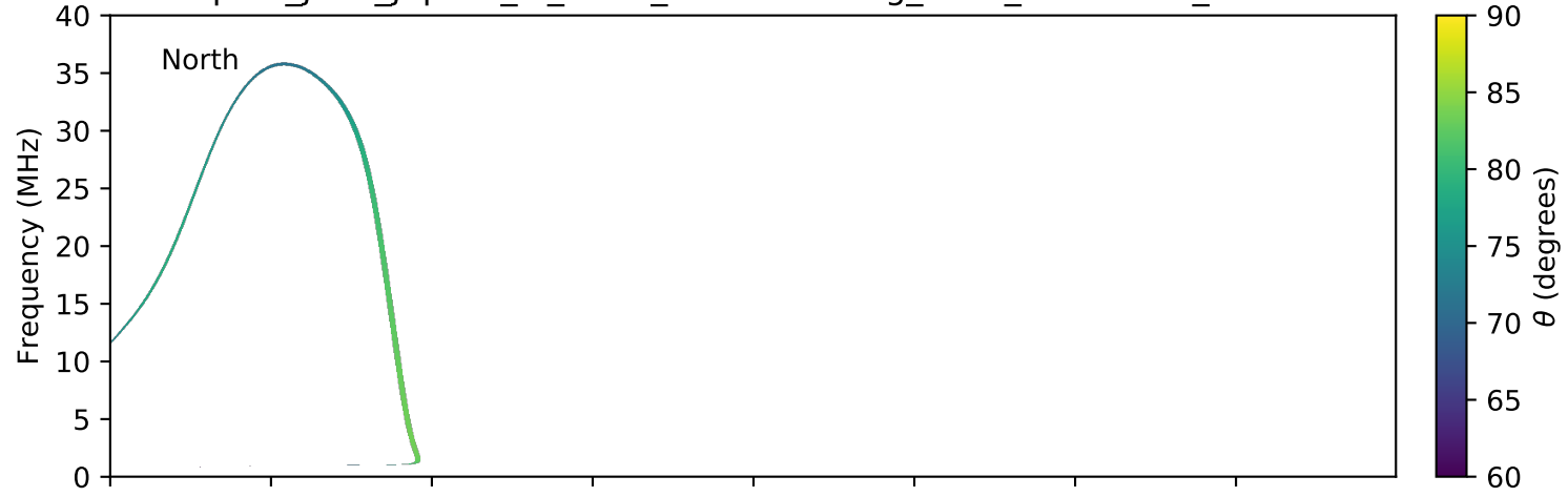
expres_juno_jupiter_io_isaac_lossc-wid1deg_3kev_20180125_v01.cdf
