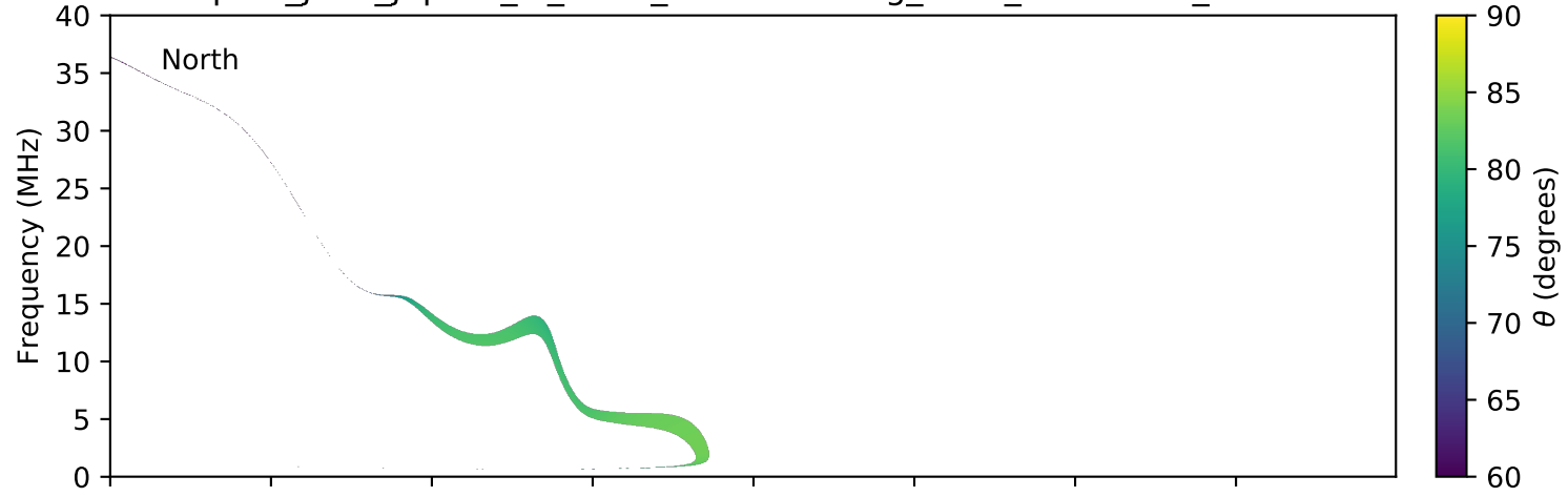
expres_juno_jupiter_io_isaac_lossc-wid1deg_3kev_20180123_v01.cdf
