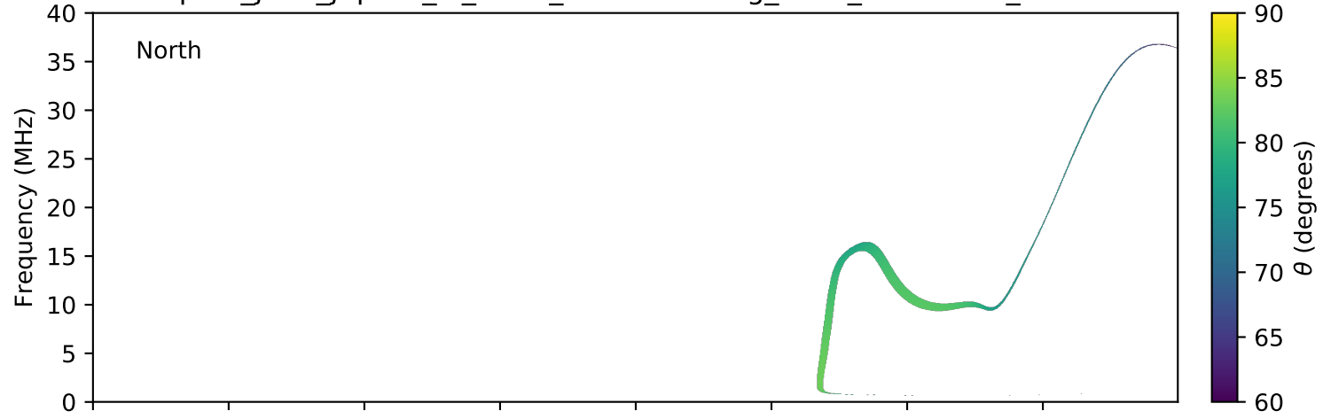
expres_juno_jupiter_io_isaac_lossc-wid1deg_3kev_20180122_v01.cdf
