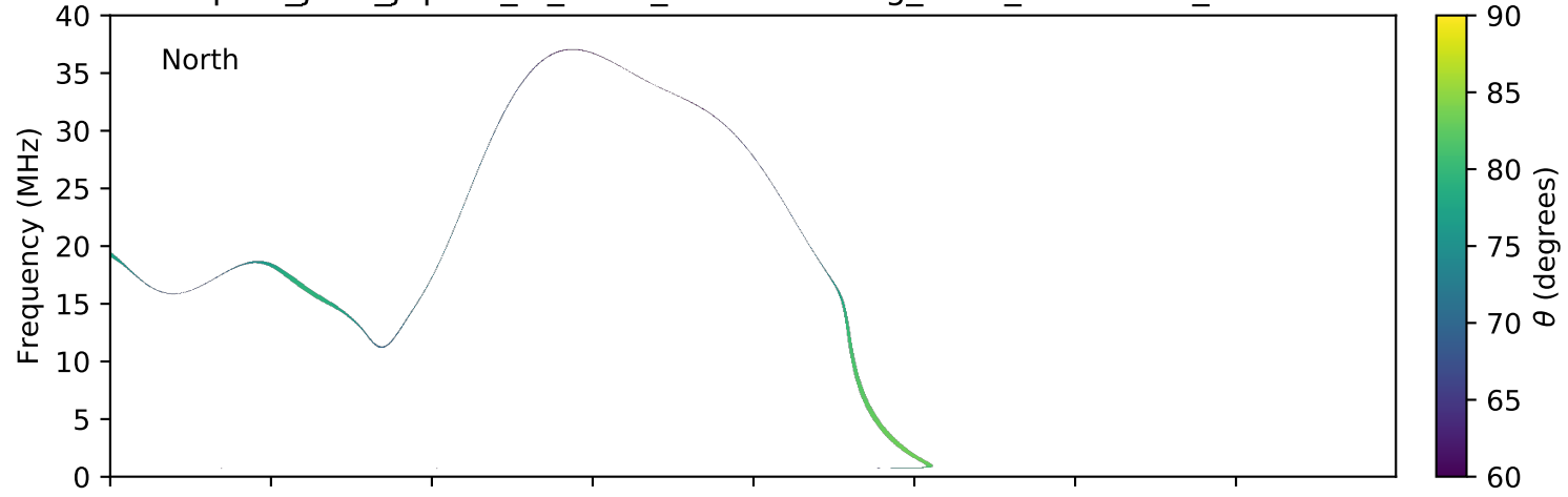
expres_juno_jupiter_io_isaac_lossc-wid1deg_3kev_20180121_v01.cdf
