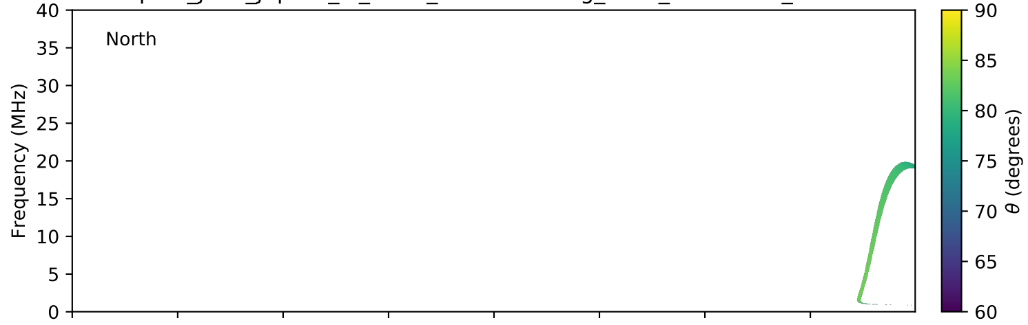
expres_juno_jupiter_io_isaac_lossc-wid1deg_3kev_20180120_v01.cdf
