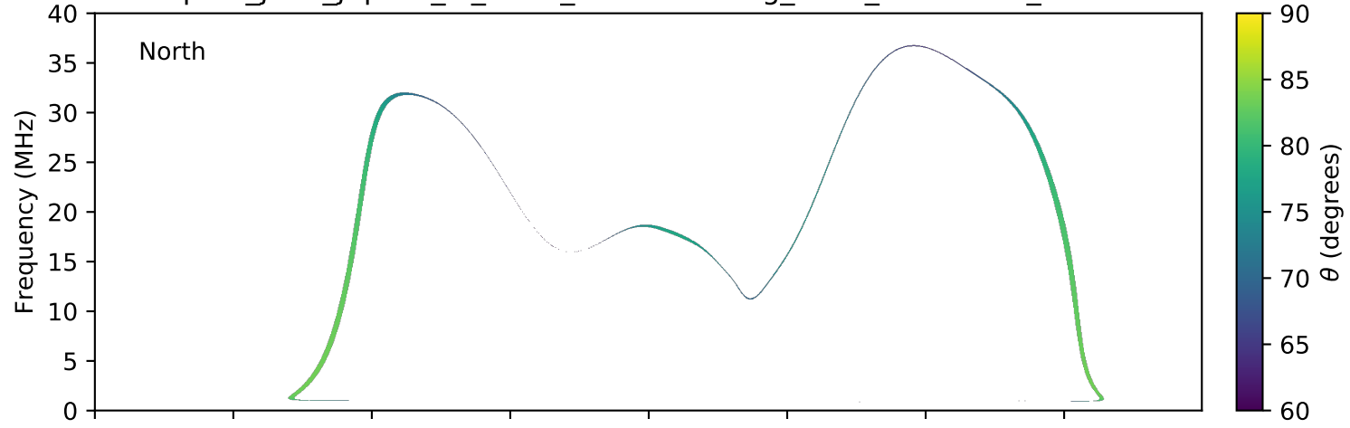
expres_juno_jupiter_io_isaac_lossc-wid1deg_3kev_20180119_v01.cdf
