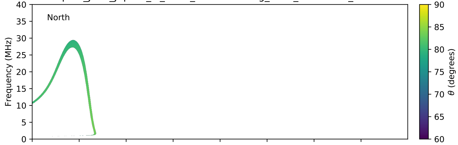
expres_juno_jupiter_io_isaac_lossc-wid1deg_3kev_20180118_v01.cdf
