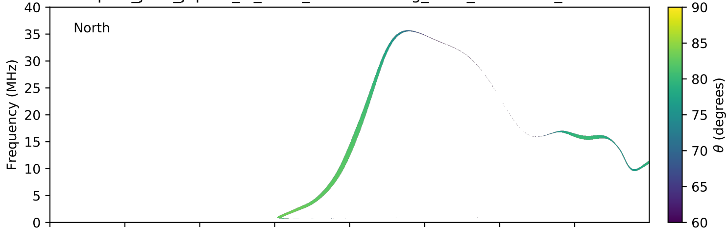
expres_juno_jupiter_io_isaac_lossc-wid1deg_3kev_20180117_v01.cdf
