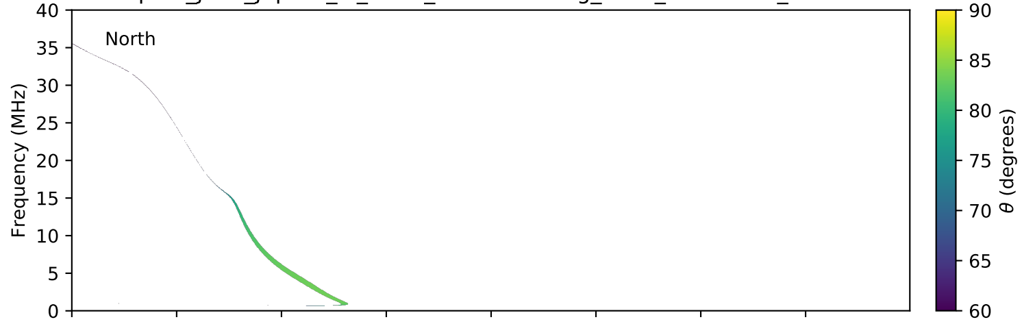
expres_juno_jupiter_io_isaac_lossc-wid1deg_3kev_20180116_v01.cdf
