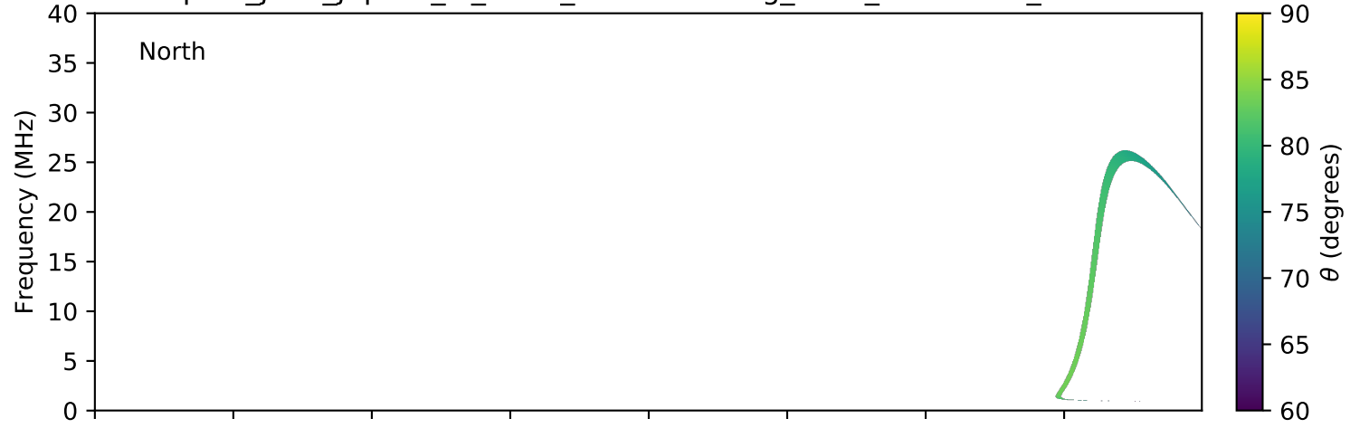
expres_juno_jupiter_io_isaac_lossc-wid1deg_3kev_20180113_v01.cdf
