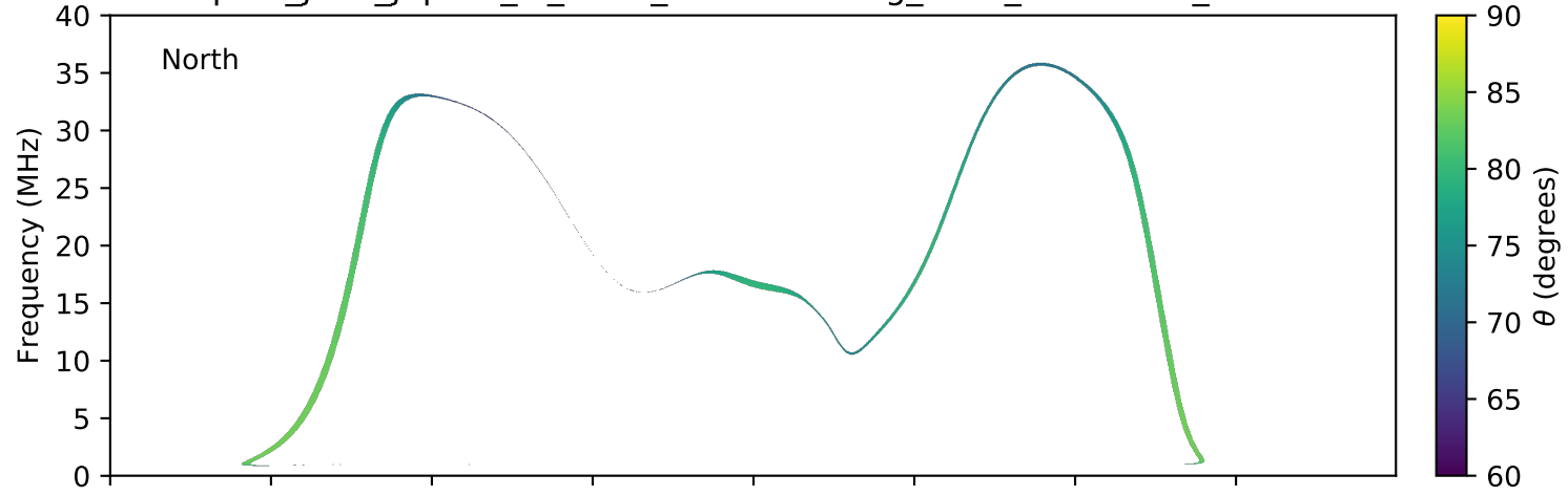
expres_juno_jupiter_io_isaac_lossc-wid1deg_3kev_20180112_v01.cdf
