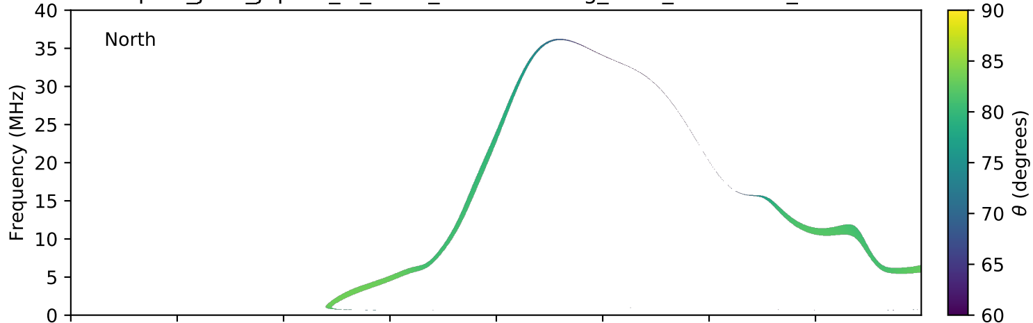
expres_juno_jupiter_io_isaac_lossc-wid1deg_3kev_20180110_v01.cdf
