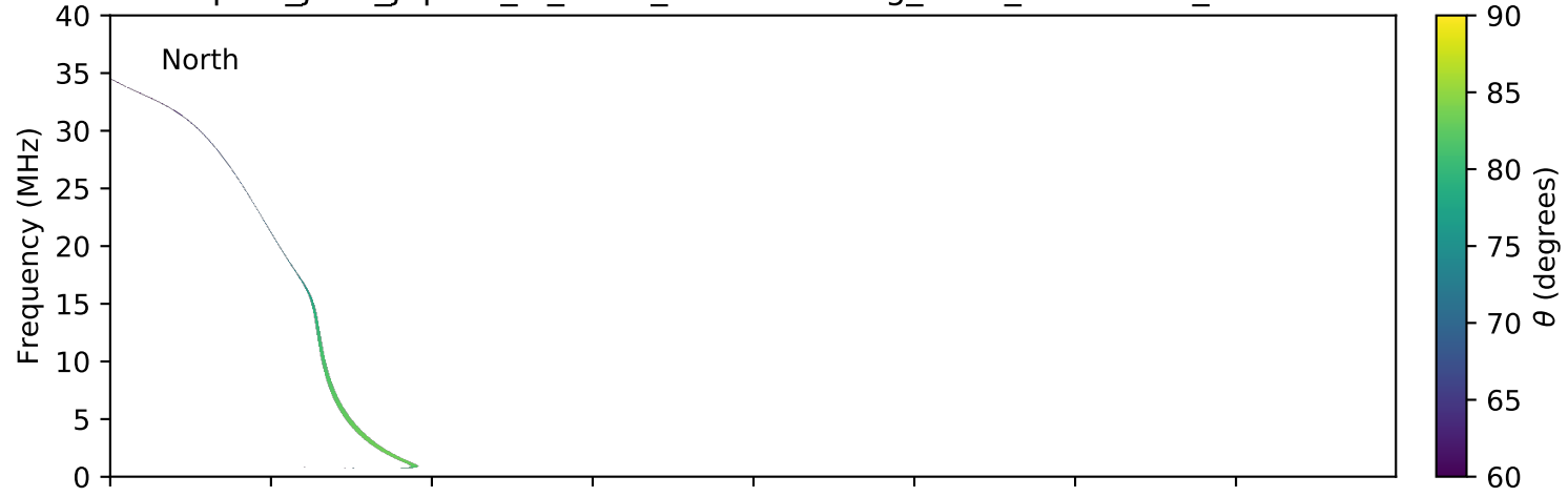
expres_juno_jupiter_io_isaac_lossc-wid1deg_3kev_20180109_v01.cdf
