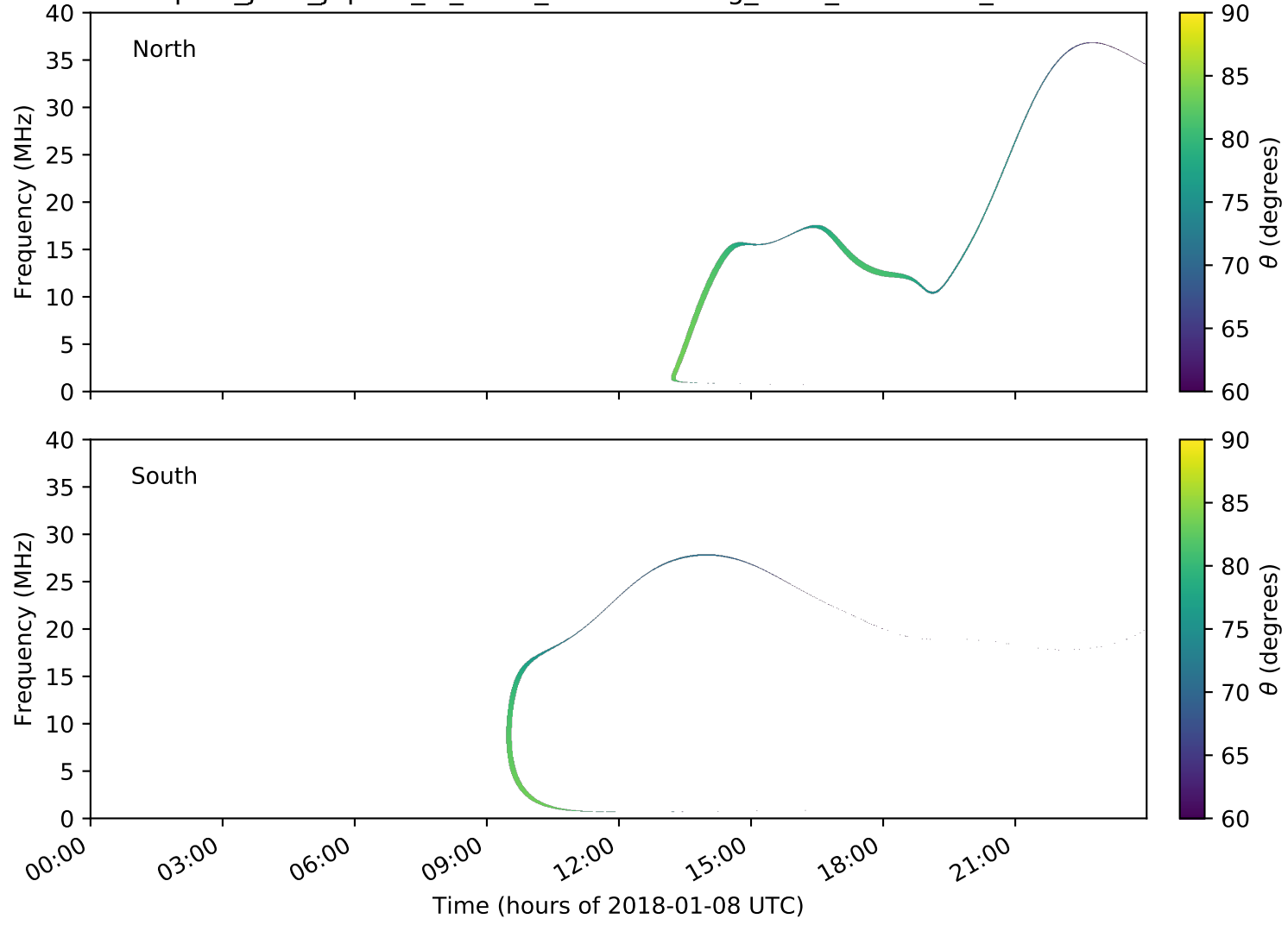
expres_juno_jupiter_io_isaac_lossc-wid1deg_3kev_20180108_v01.cdf
