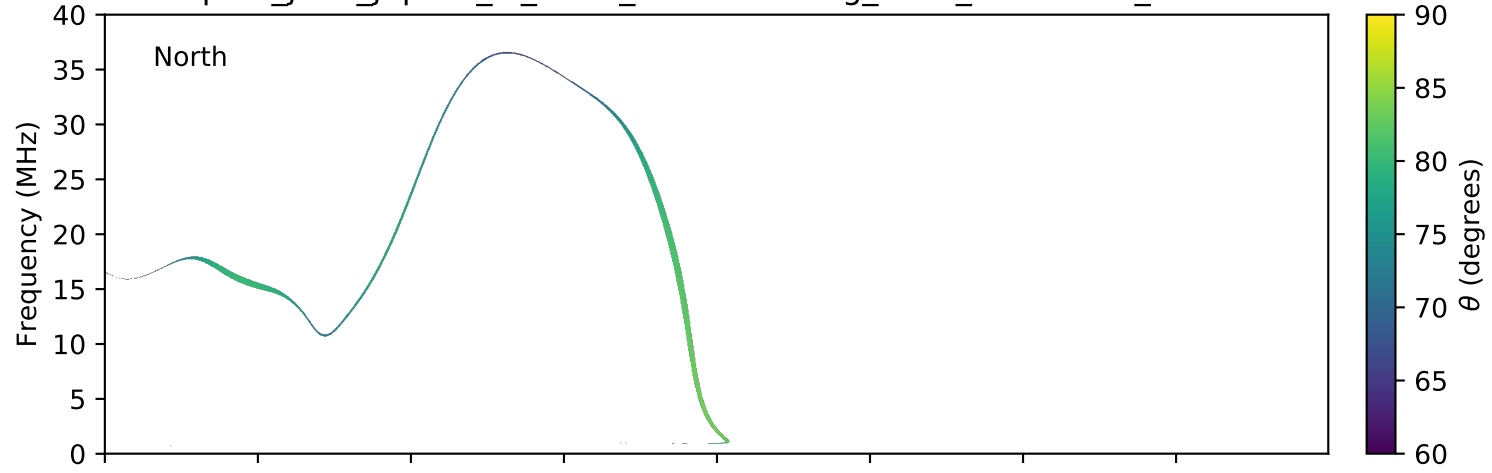
expres_juno_jupiter_io_isaac_lossc-wid1deg_3kev_20180107_v01.cdf
