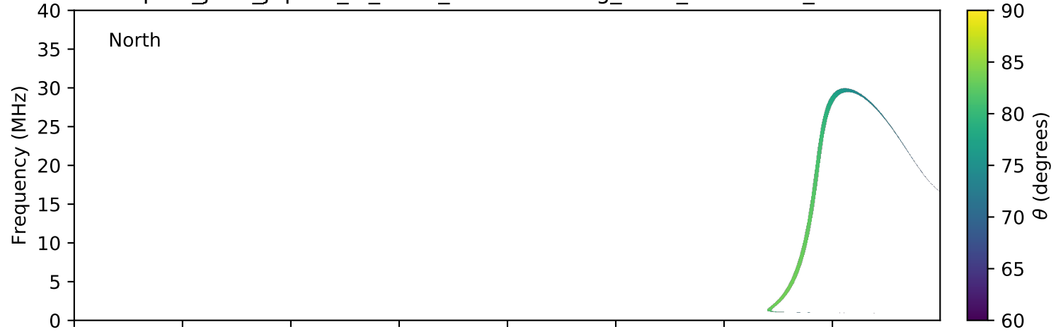
expres_juno_jupiter_io_isaac_lossc-wid1deg_3kev_20180106_v01.cdf
