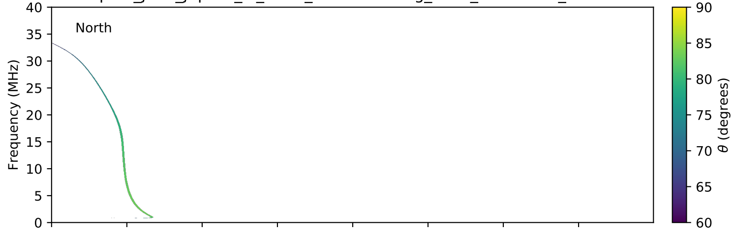
expres_juno_jupiter_io_isaac_lossc-wid1deg_3kev_20180102_v01.cdf
