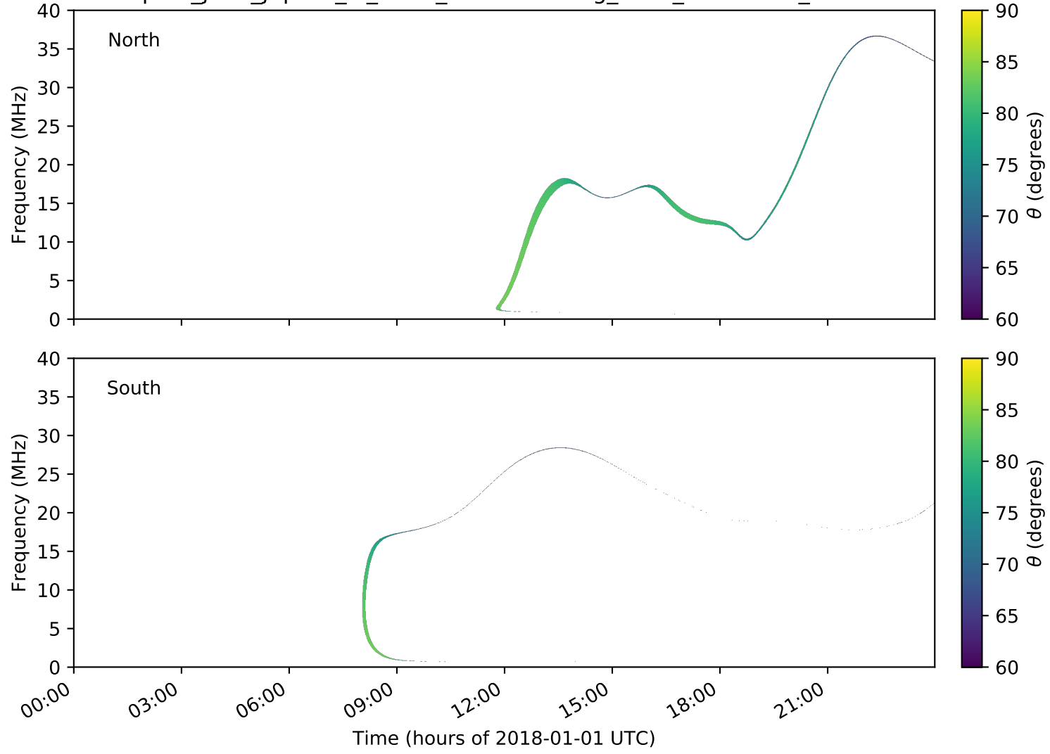
expres_juno_jupiter_io_isaac_lossc-wid1deg_3kev_20180101_v01.cdf
