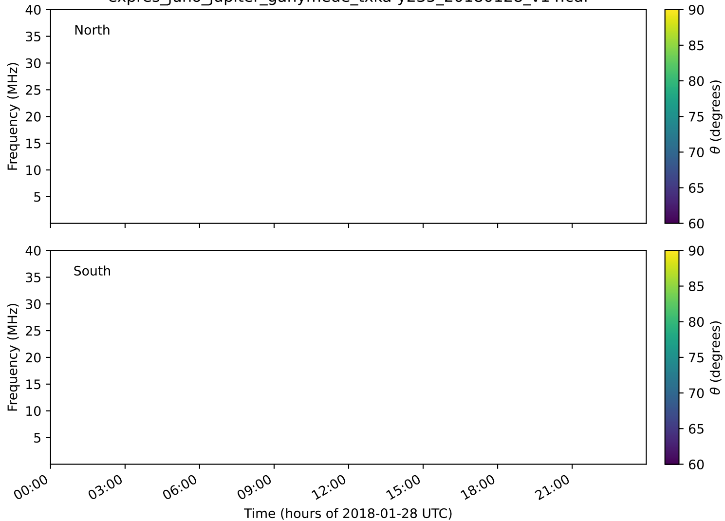
expres_juno_jupiter_ganymede_txka-y235_20180128_v14.cdf
