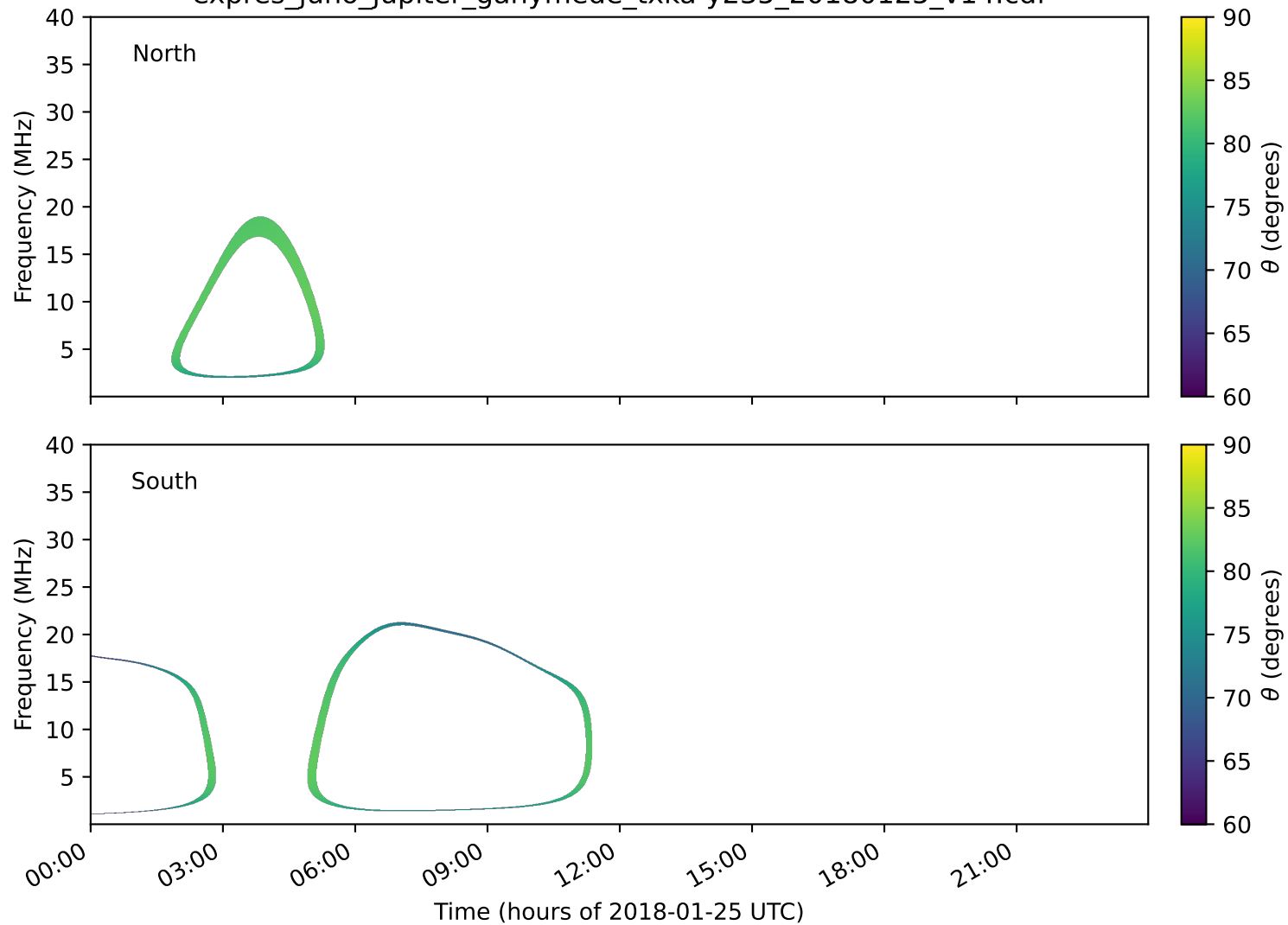
expres_juno_jupiter_ganymede_txka-y235_20180125_v14.cdf
