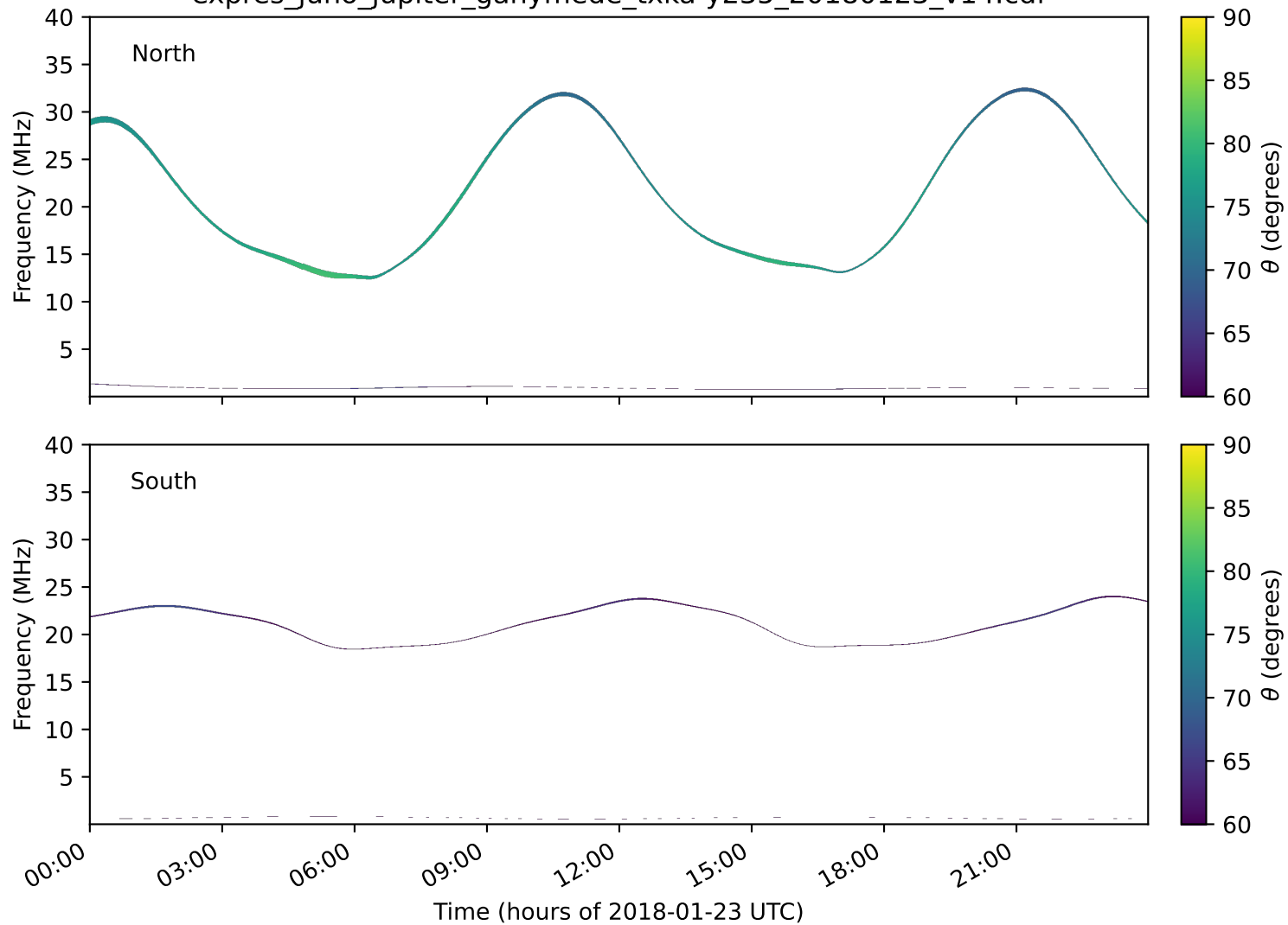
expres_juno_jupiter_ganymede_txka-y235_20180123_v14.cdf
