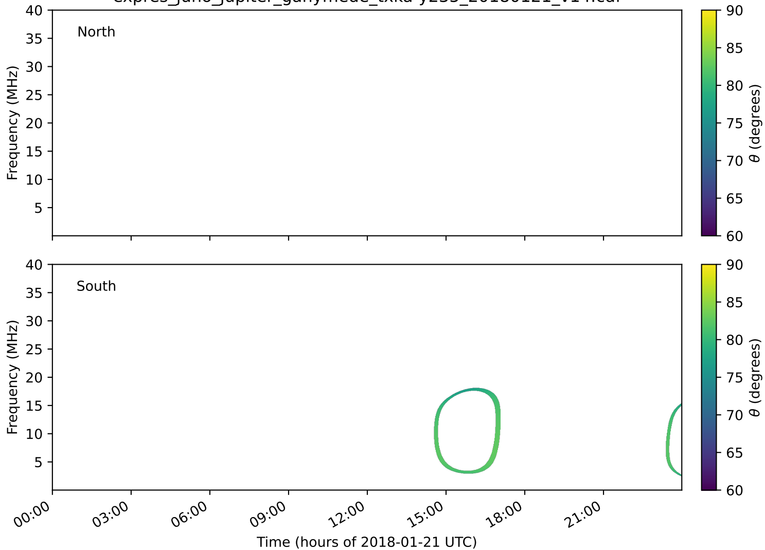
expres_juno_jupiter_ganymede_txka-y235_20180121_v14.cdf
