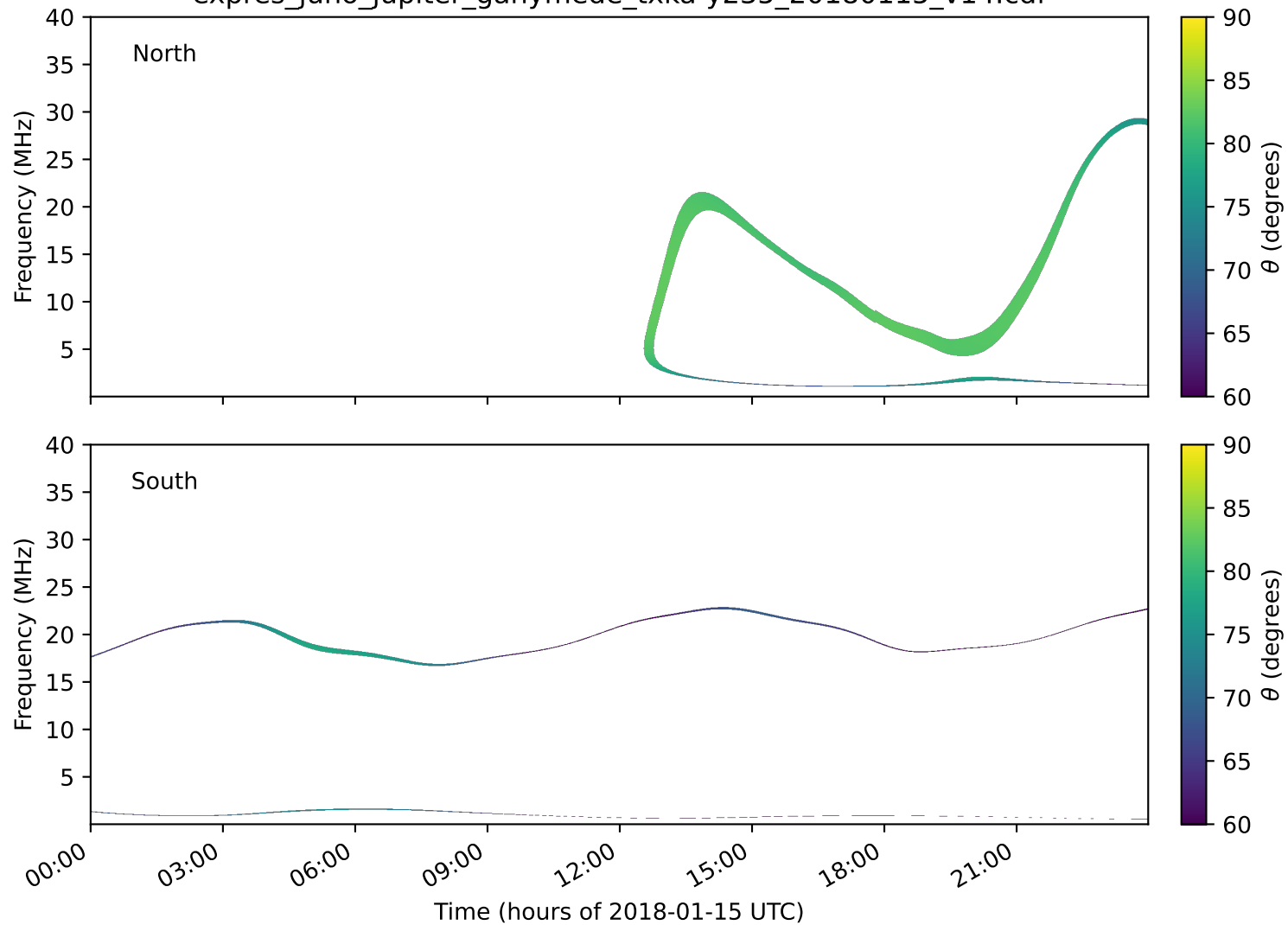
expres_juno_jupiter_ganymede_txka-y235_20180115_v14.cdf
