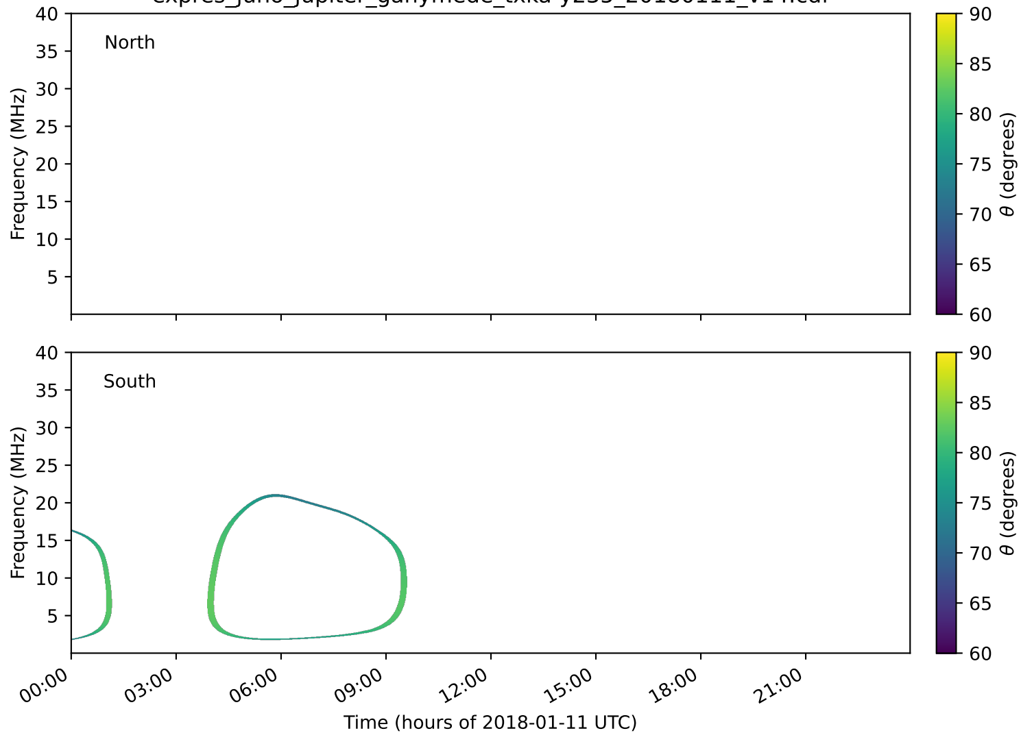
expres_juno_jupiter_ganymede_txka-y235_20180111_v14.cdf
