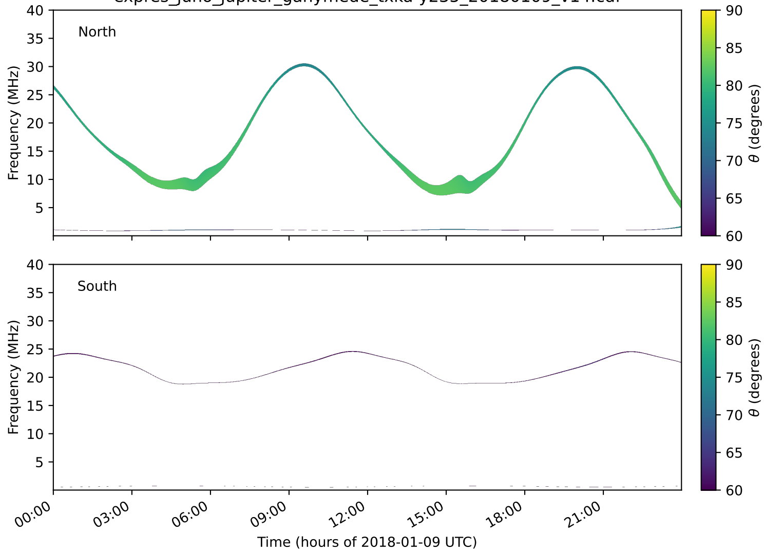
expres_juno_jupiter_ganymede_txka-y235_20180109_v14.cdf
