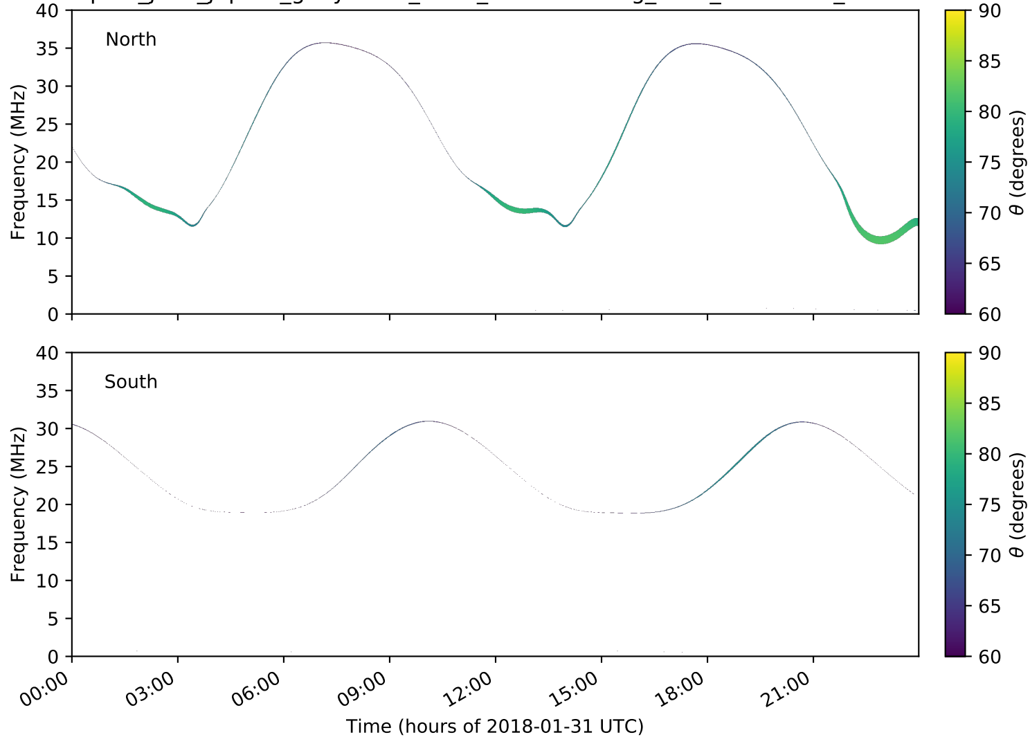
expres_juno_jupiter_ganymede_isaac_lossc-wid1deg_3kev_20180131_v01.cdf
