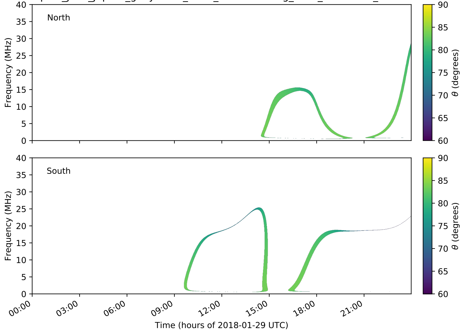
expres_juno_jupiter_ganymede_isaac_lossc-wid1deg_3kev_20180129_v01.cdf
