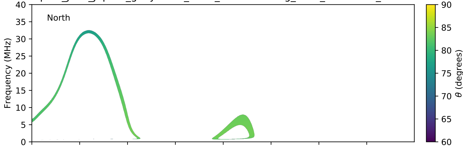
expres_juno_jupiter_ganymede_isaac_lossc-wid1deg_3kev_20180125_v01.cdf
