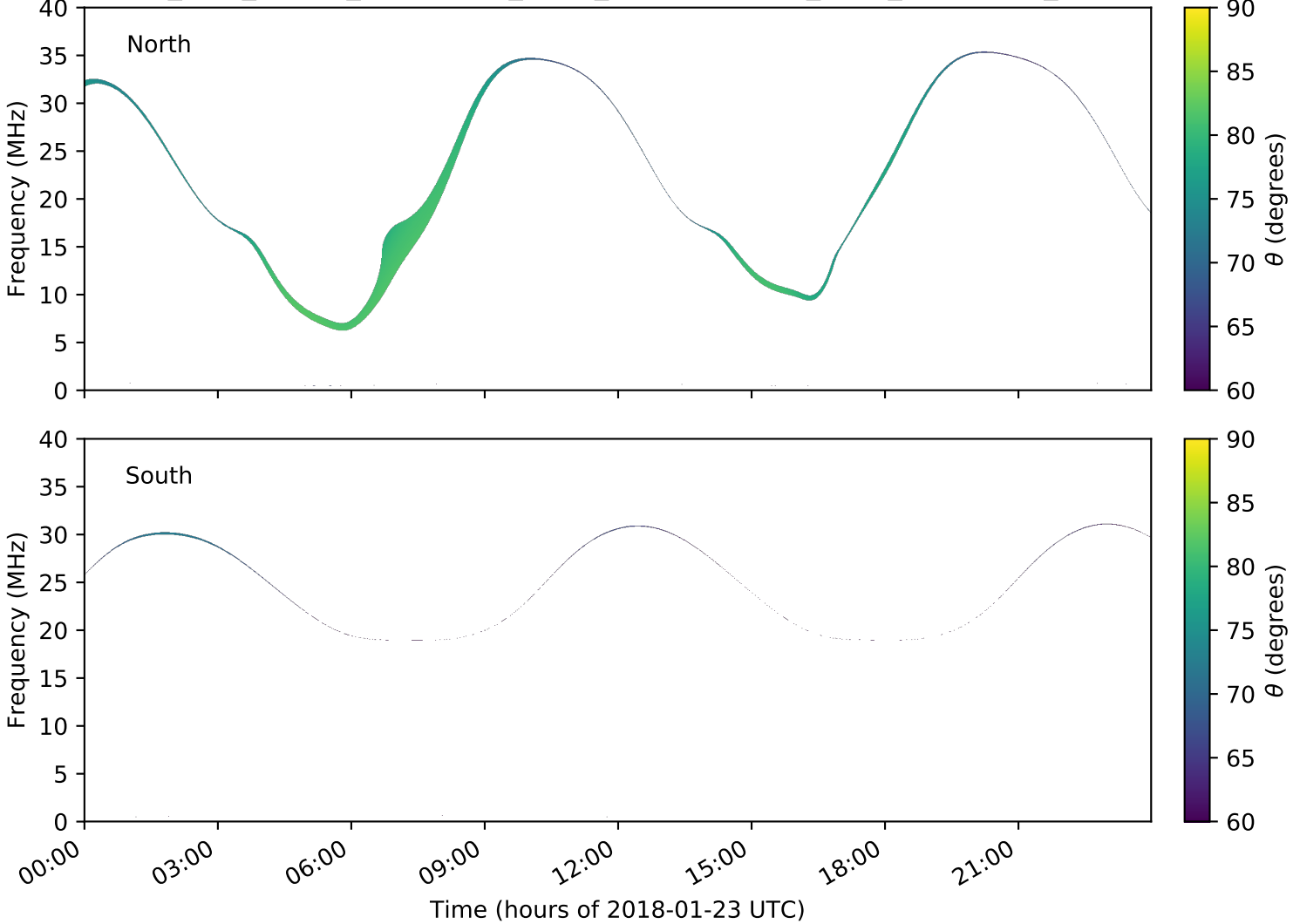
expres_juno_jupiter_ganymede_isaac_lossc-wid1deg_3kev_20180123_v01.cdf
